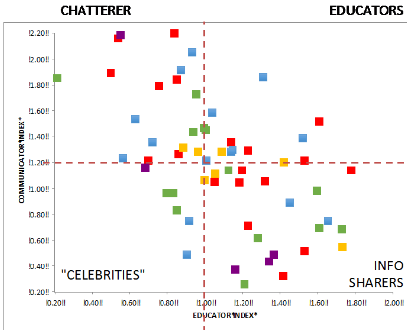
Figure 2 Candidate Segmentation
